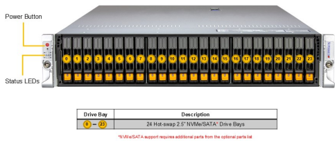
(Front View – System) Optional Configuration
