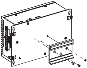
DIN-Rail Assembly
