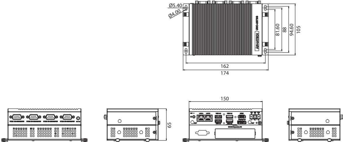
Double stack with with UNO-2372G-EKCE
